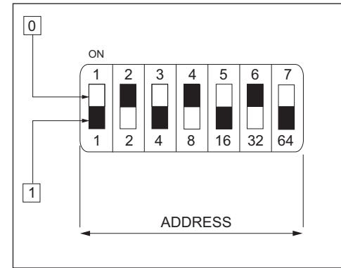
Fig 3. DIL Switch
