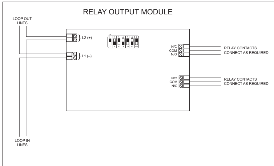
Fig 2. Wiring Diagram for Alpha Relay Output Module
